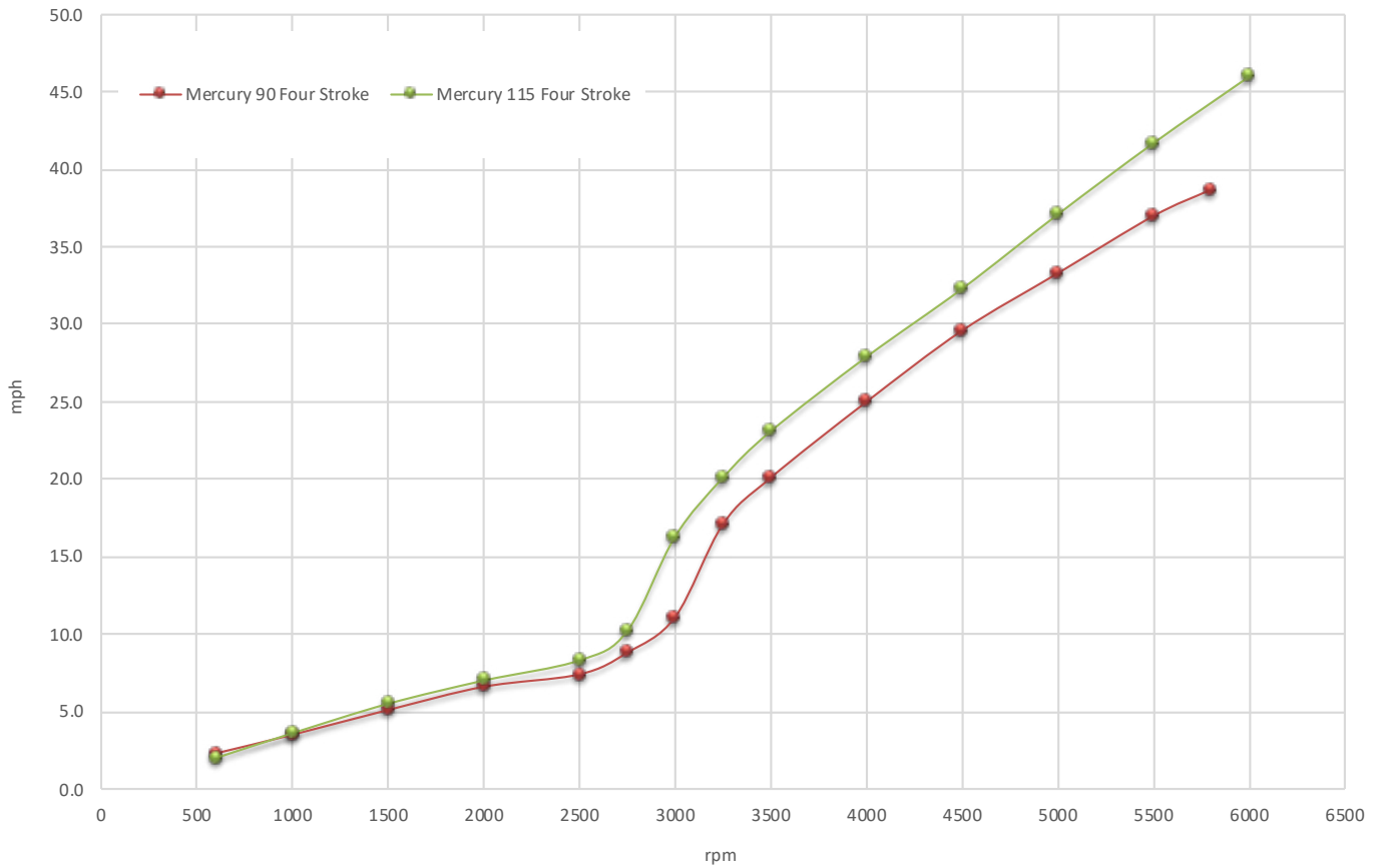
170 Montauk 2018 Engine Comparison Graph
